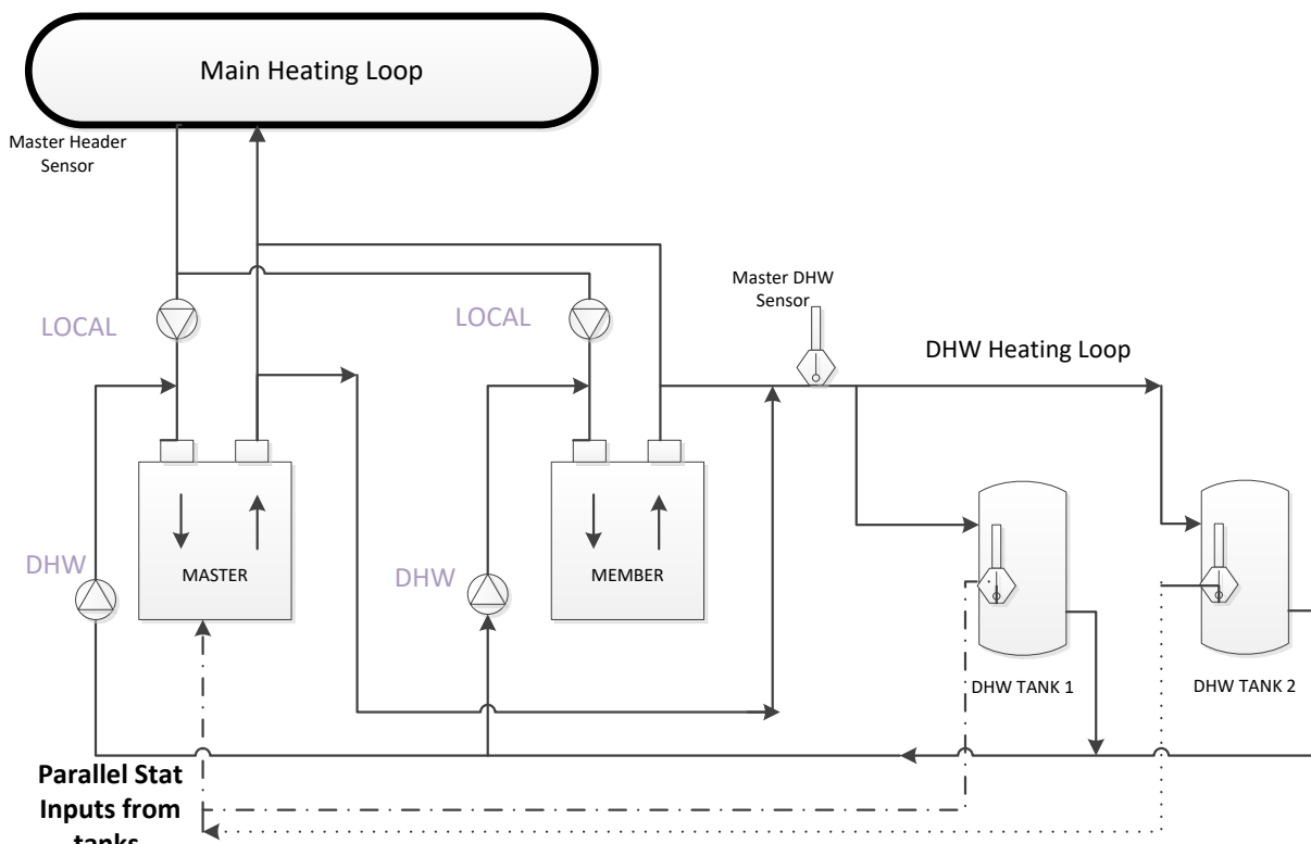
Simplified Drawing 1.
